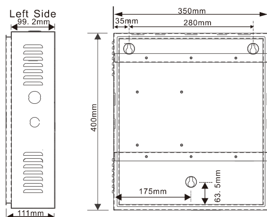
Figure 1. Installation Dimension of Panel
