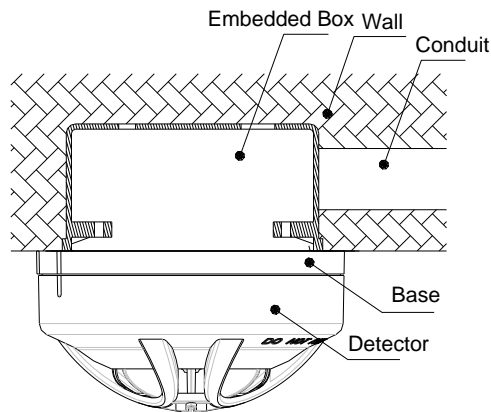
Fig.3: TX3110 Installation Drawing
