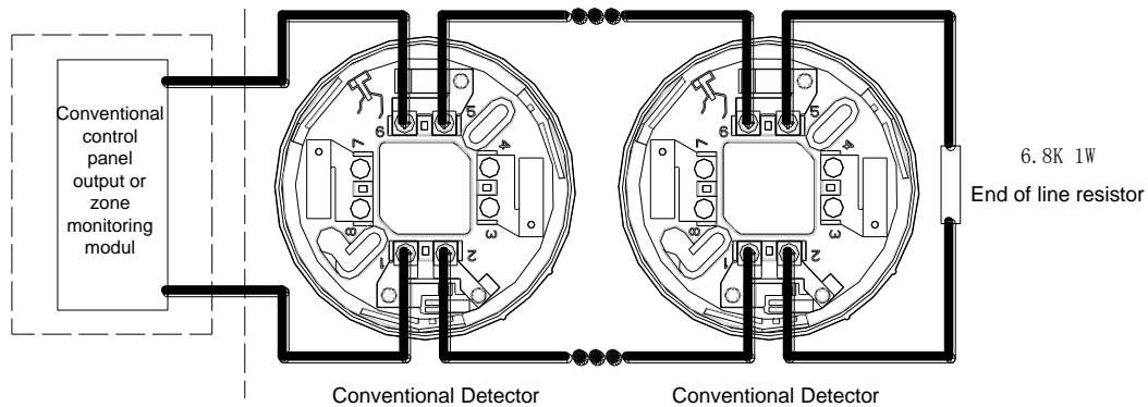
Fig 5: Multiple TXC3110 Wiring
