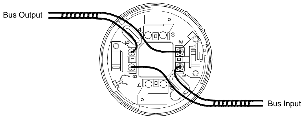
Fig.4: Single TXC3110 Wiring
